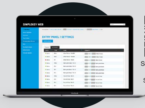
EV6
